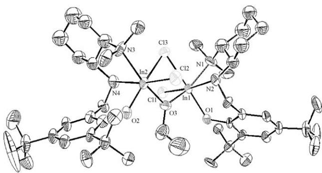
Figure 1. Molecular structure of 1 with thermal ellipsoids set at 35% probability. Hydrogen atoms are omitted for clarity.
